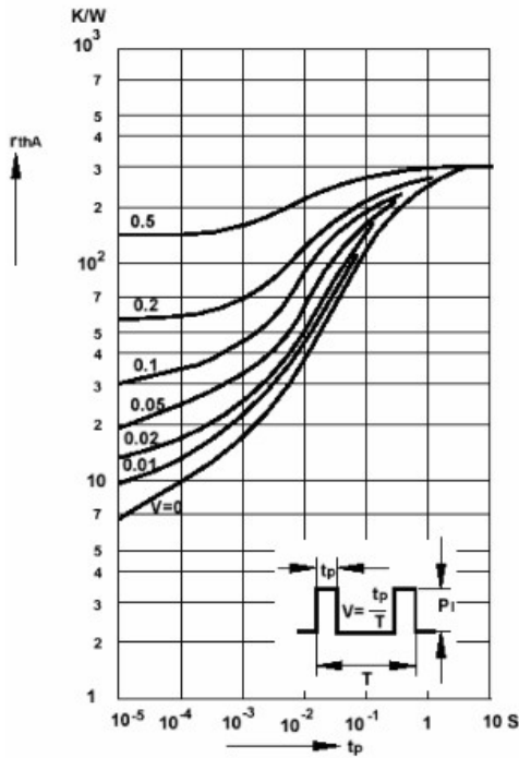
Pulse thermal resistance versus pulse duration
